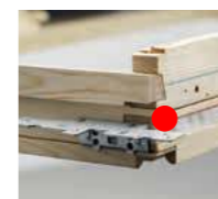
0 level height – install the brackets at top and bottom of frame at red line to use with EDW/EDL flashings.
