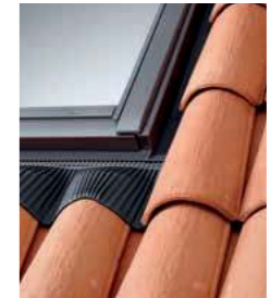
EDW Flashing High-profiled roofing material up to 120 mm
