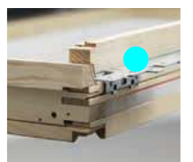
-40 mm level height – install the brackets at the sides of the frame at blue line to use with EDJ/EDN flashings
